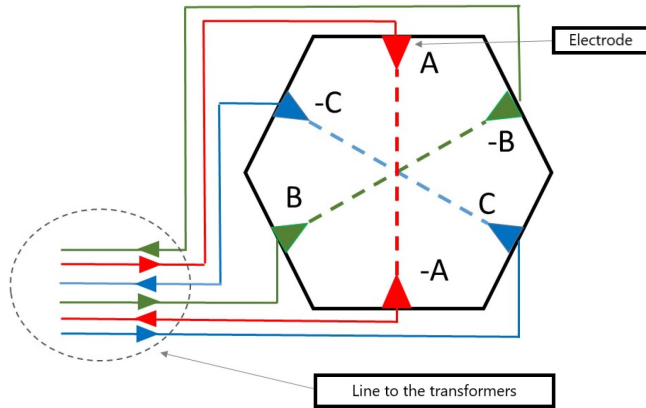
FIGURE 1. Circuit diagram of electric currents.
