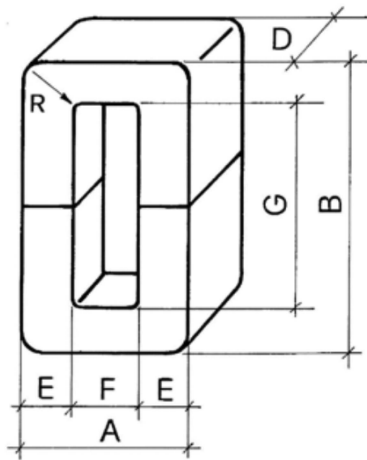
FIGURE 10. Diagram of the magnetic core of shield source coupling with indication of the dimensions.
