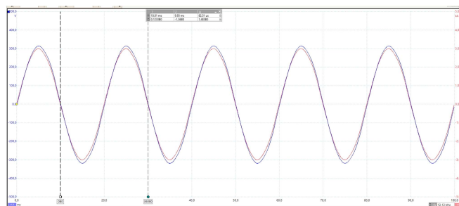
FIGURE 17. Phase "A" voltage and current measured at the electrodes.
