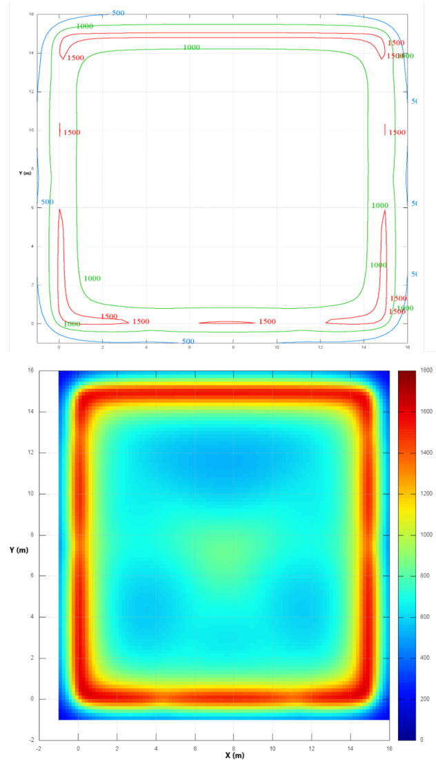
FIGURE 5. Isopleth lines and chromatic map of magnetic induction on a horizontal surface placed under the furnace.
