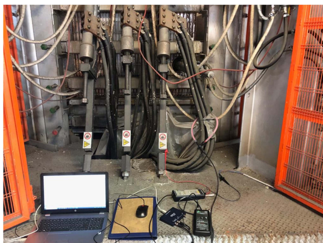
FIGURE 15. Instrumentation connected to the electrodes: measurement of the current circulating in a single electrode.
