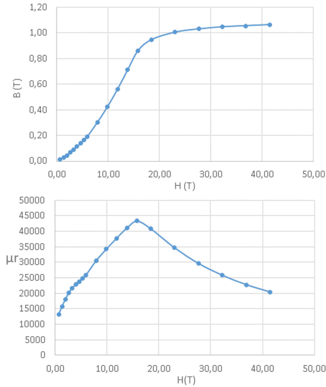
FIGURE 12. Magnetic characteristic and relative permeability of the closed core.
