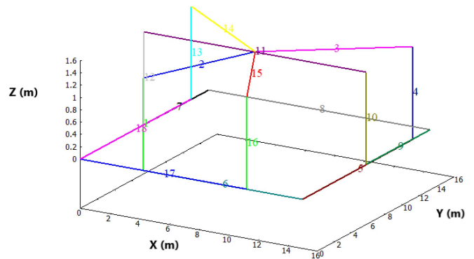
FIGURE 3. Filiform model of the electrical connections around the furnace and of the current inside the glass.
