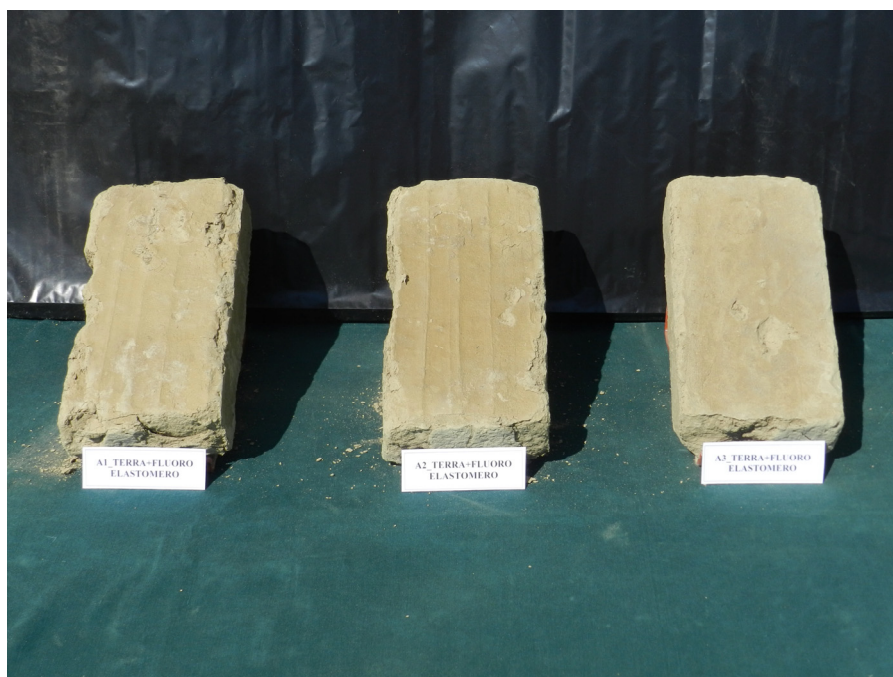
Figure 5. Earthen bricks: Specimens made with local earth (from Alessandria, Italy) and treated with a fluoroe elastomer (Tecnoflon N215).
