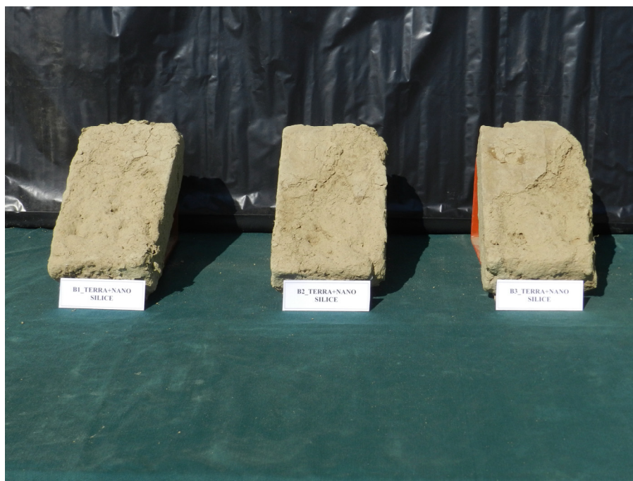
Figure 6. Earthen bricks: Specimens made with local earth (from Alessandria, Italy) and treated with nano-silica (Nano Estel).
