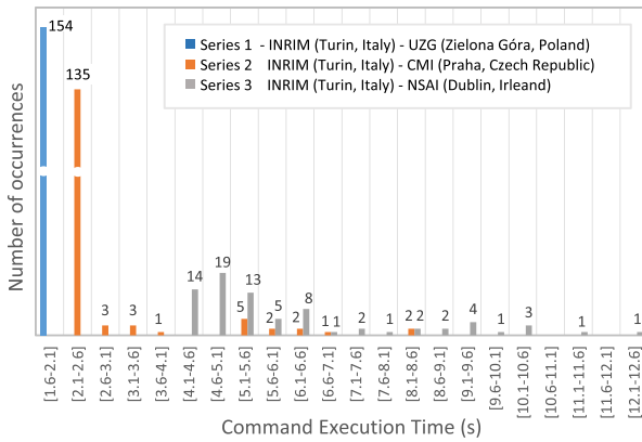
Fig. 14. Histograms of DSS-2A command execution times in the remote-control on long distance (public institutions).
