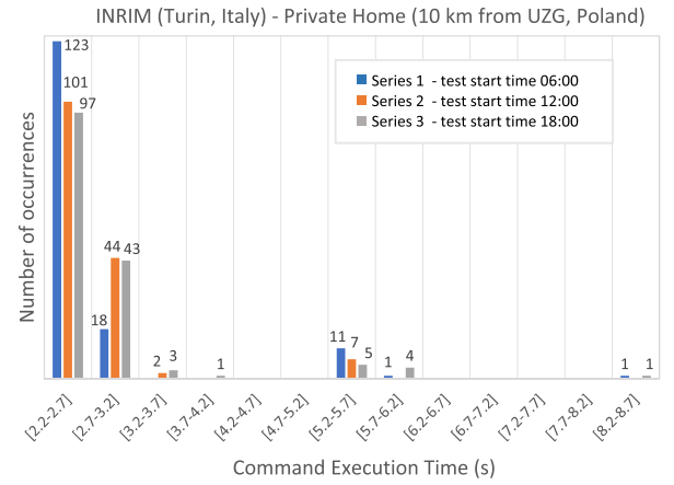
Fig. 15. Histograms of DSS-2A command execution times in the remote-control on long distance (private home).
