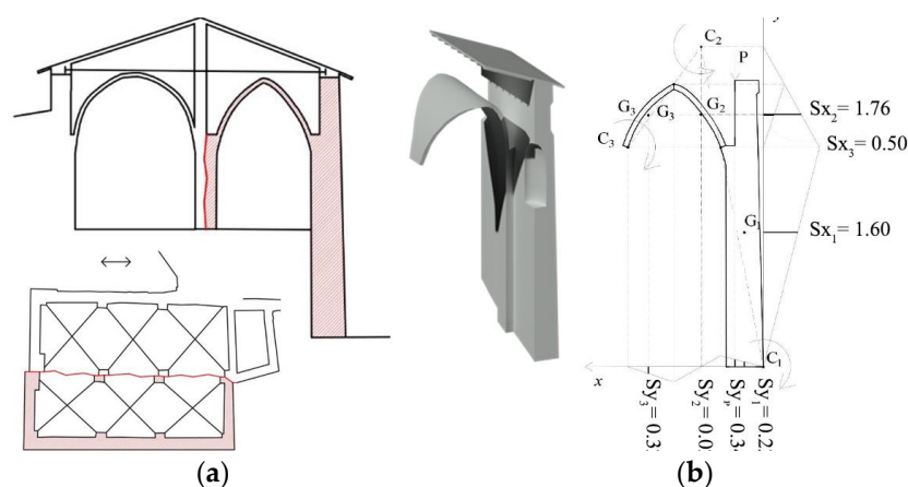
Figure 16. Representation of the wall mechanism: (a) 2D and 3D model extrapolated from the simplified volumetric; and (b) analysis of the south side wall, with graphical solution of the equilibrium conditions analysis for the calculation of the seismic coefficient.
