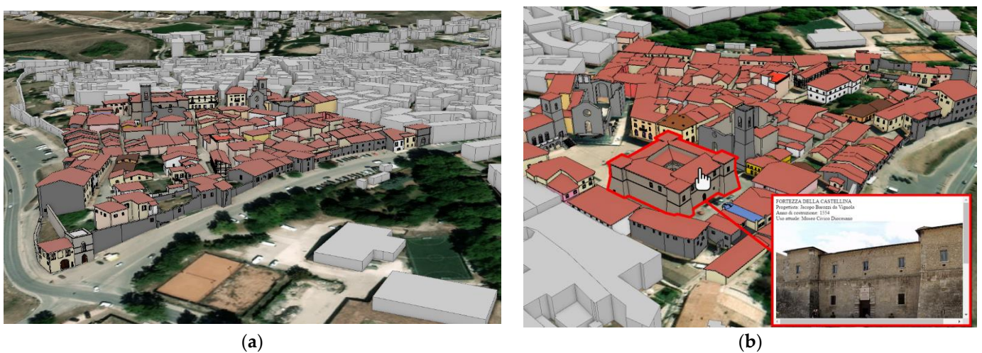
Figure 12. The Urban BIM related to Norcia city centre: the south-west part of the city (a), with a zoomed view on the Castellina 3D model and query in the 3D database (b).
