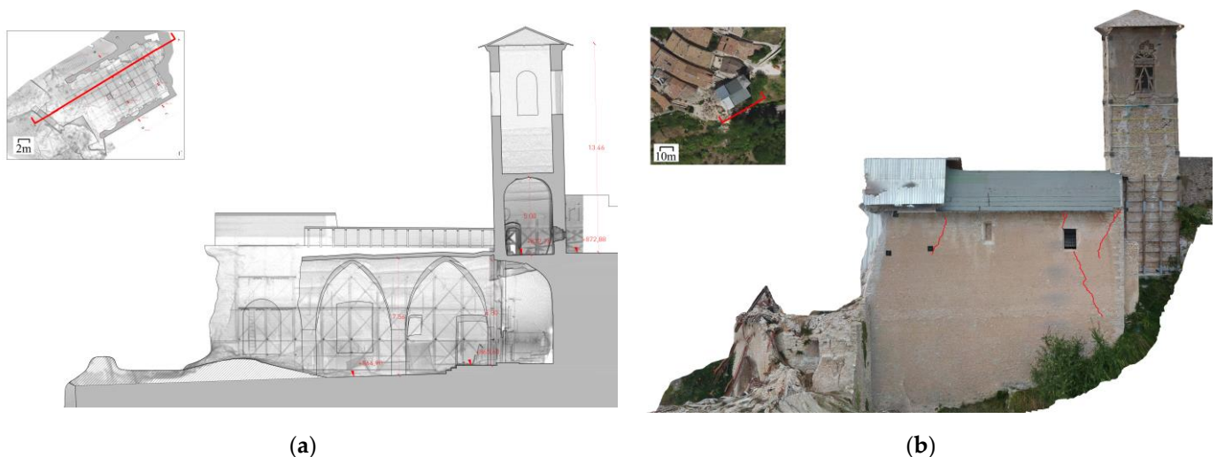
Figure 9. Examples of 2D digital products: (a) section; and (b) façade orthophoto for the Sant'Andrea.
