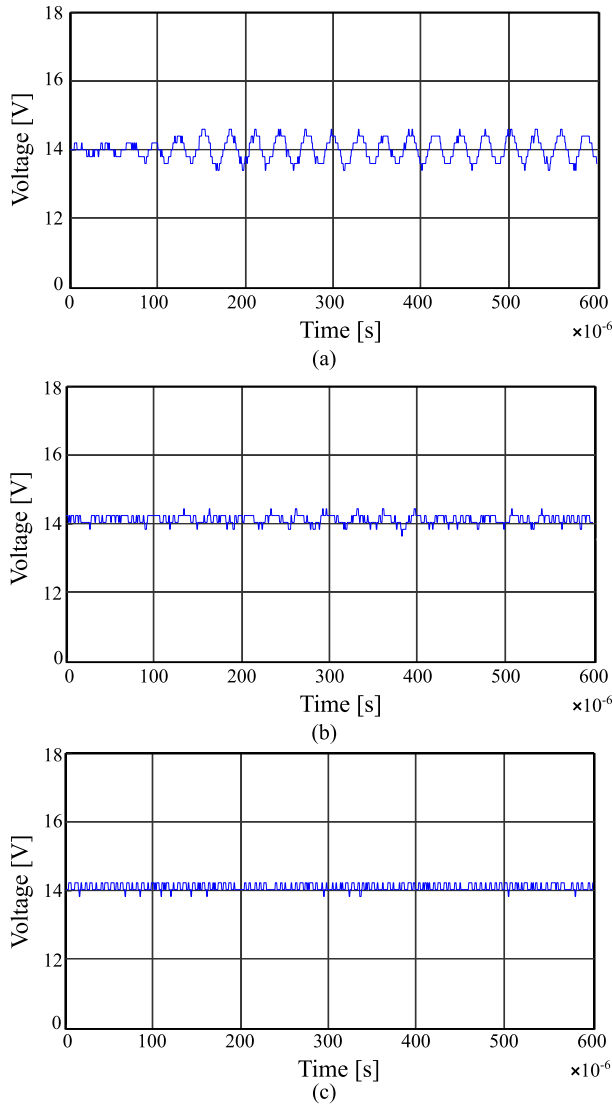
FIGURE 13. Measured output voltage of the boost converter. (a) N_{ADC} = 7 , N_{DPWM} = 5 ; (b) N_{ADC} = 7 , N_{DPWM} = 5 , N_{DDPM} = 4 ; (c) N_{ADC} = 7 , N_{DPWM} = 5 , N_{DDPM} = 4 .
