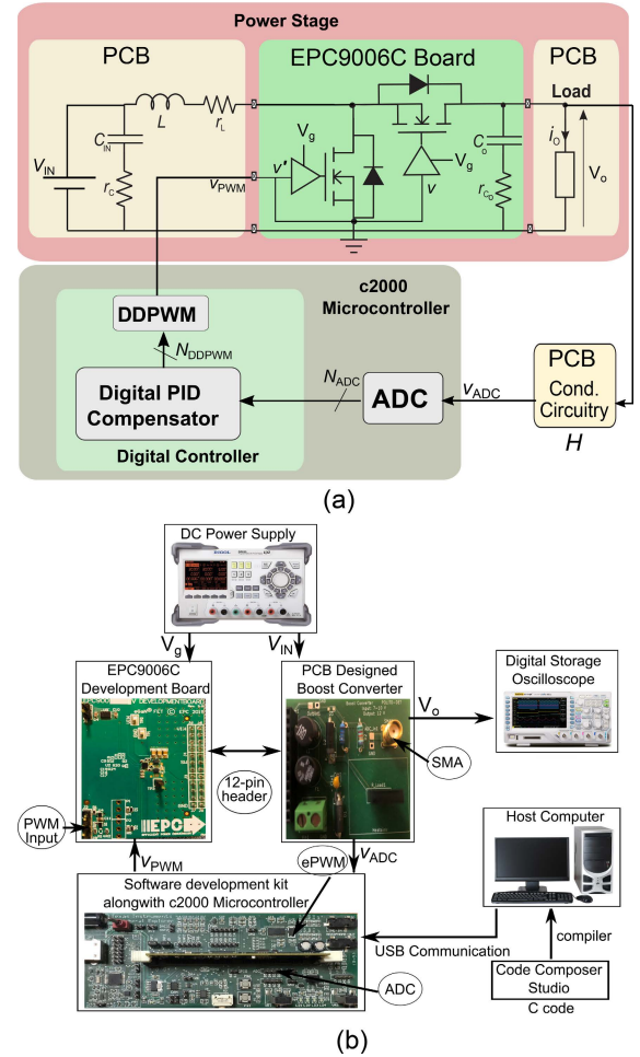
FIGURE 10. Experimental test setup of digitally controlled boost converter (a) Test setup schematic (b) Block diagram of the experimental testbench.
