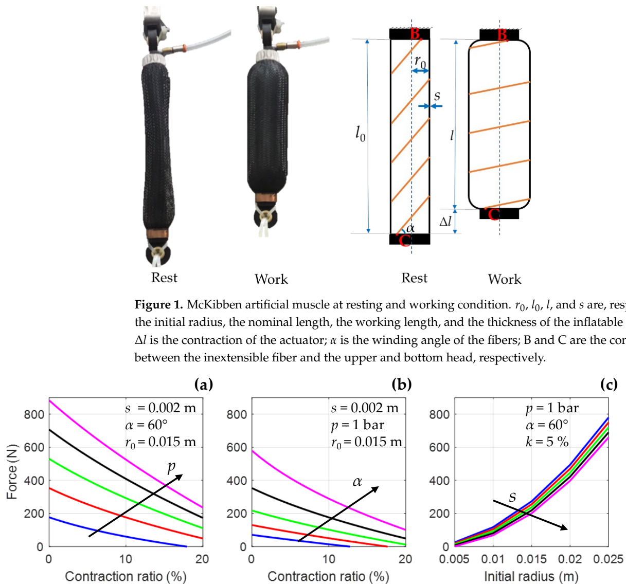
Figure 2. Traction force of McKibben's muscle for different geometrical and functional parameters. (a) The MKM tensile force for different supply pressure p [0.5; 1; 1.5; 2; 2.5] bar; (b) The MKM tensile force for different winding angle \alpha of the inextensible fibers [45; 50; 55; 60; 65]°; (c) The MKM tensile force for different thickness s of the inflatable chamber [1; 2; 3; 4; 5] mm. The nominal length has been set to 0.2 m for all simulations. In the graph r_0 is the resting radius; k is the contraction ratio.
