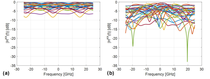
Fig. 4. 30 realizations of the H^{xx}(f) transfer function for one of the 300 configurations of a 25 GBaud 220 m OM3-based Coh-MMF system with a) no MMF connectors or b) 4 MMF connectors.
