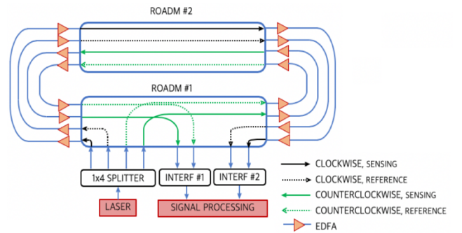
Fig. 9. Application of the proposed sensing architecture in a ring network in presence of ROADMs.
