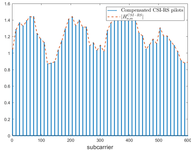
Figure 2. Module of interpolated channel matrix |H_{n,m}^{CSI-RS}| .
