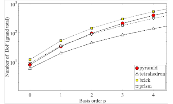
Fig. 4. Total number of degrees of freedom (DoF) for curl-conforming vector bases of order p on single, differently shaped canonical cells.
