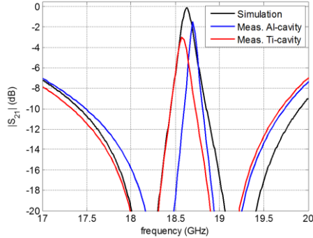
Fig. 5 Comparison between simulated (black line) and measured transmission coefficients of the test cavities in AlSi10Mg and Ti6Al4V (blue and red lines, respectively).
