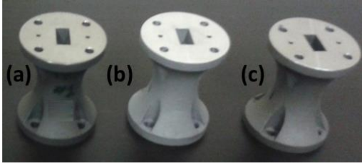
Fig. 10 Sixth-order stop-band filter prototypes with optimized design for the SLM process. (a) AlSi10Mg alloy. (b) Ti6Al4V alloy. (c) Maraging steel.
