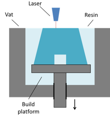
Fig. 3 Vat photo-polymerization process (e.g., stereolithography).
