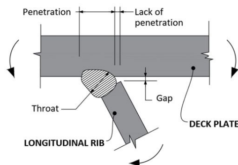
Figure 3. Rib-deck connection [46].
