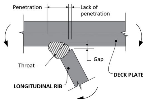
Figure 3. Rib-deck connection [46].
