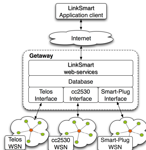
Fig. 1. Software infrastructure scheme to handle heterogeneous wireless sensor networks.
