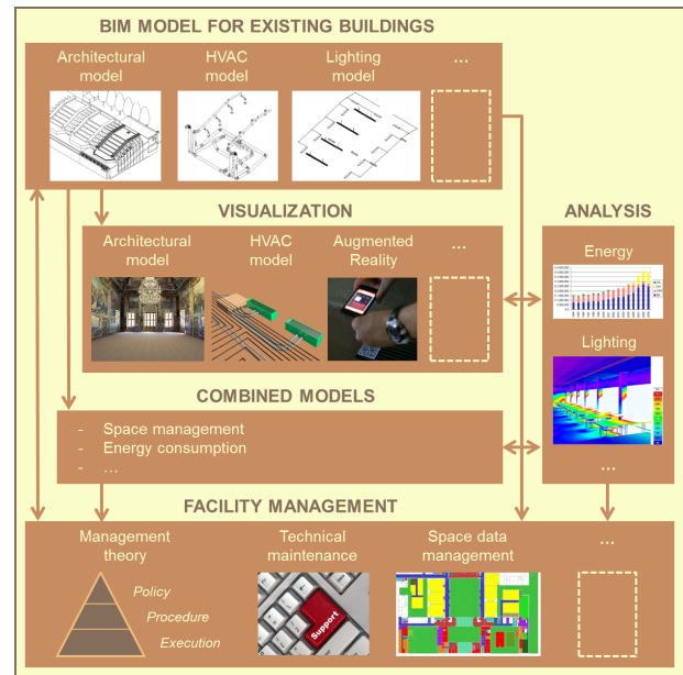
Fig. 2. Data management structure on a Building Information Modelling architecture.
