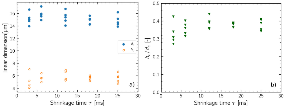
Fig. 4. Values of crust thickness h_c , granule diameter d_c and h_c/d_c ratio for clusters obtained at high Péclet number at varying evaporation time \tau . For every \tau , five different but equivalent simulations were run. The cluster morphology is not significantly affected by the shrinkage time in the high Péclet number regime.
