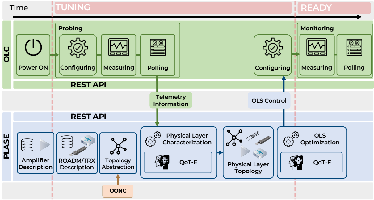
Fig. 2. Qualitative time line of the proposed cognitive optical control plane operation that leads an OLS to be ready for use.
