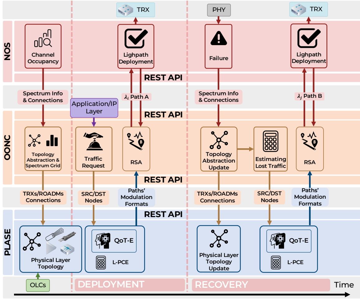
Fig. 3. Qualitative time line of the proposed optical data plane operation: establishment of a connection following a LP request and a recovery after a failure detection.
