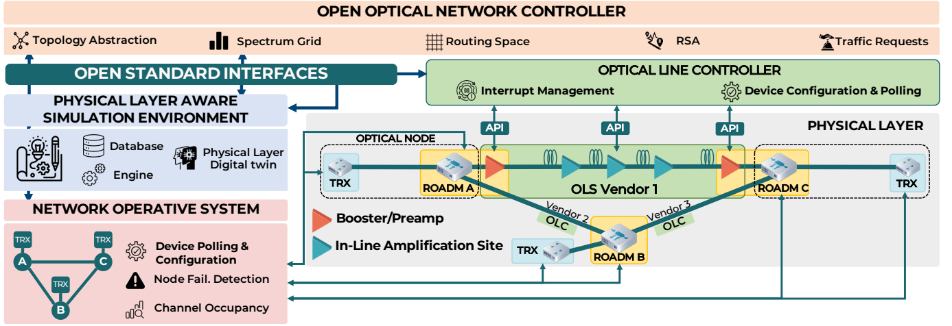
Fig. 1. Abstract scheme of the open and disaggregated optical network architecture, designed to independently manage the optical data and control plane.
