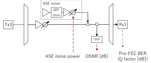
Fig. 2: Evaluation setup to obtain \text{SNR}_{\text{res}}
