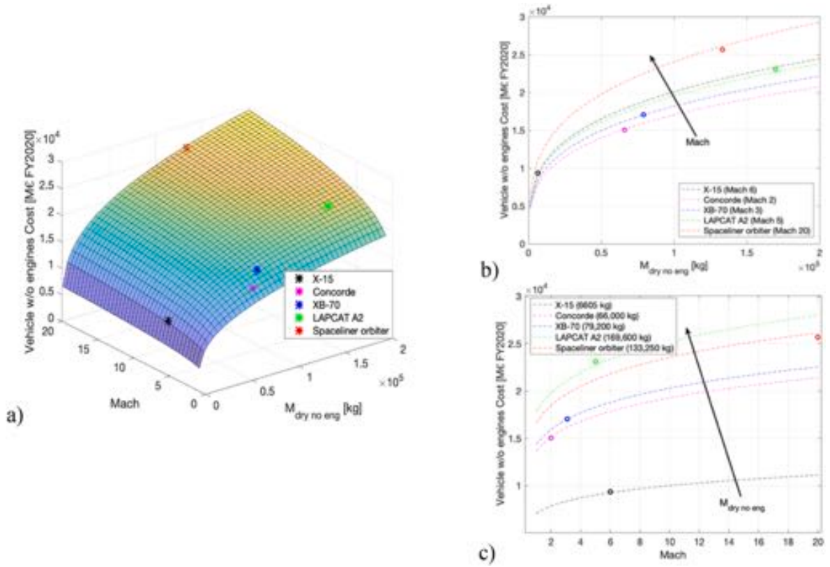
Fig. 4. a) 3D Construction of the Vehicle (w/o Engine) RDTE CER (Eq. (2)) with a hypersonic dataset; b) 2D Variation of the Vehicle (w/o Engine) Cost as function of the vehicle dry mass (w/o Engine) using Mach number as parameter; c) 2D Variation of the Vehicle (w/o Engine) Cost as function of the Mach number using vehicle dry mass (w/o Engine) as parameter.
