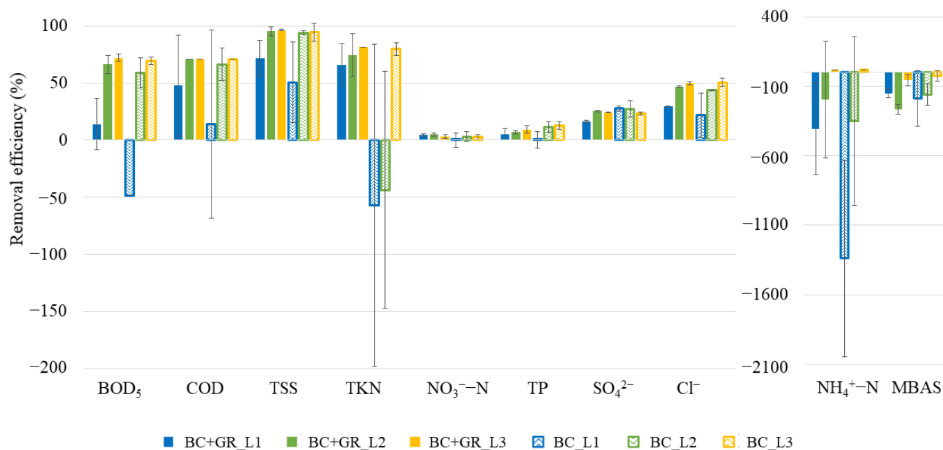
Figure 5. Removal efficiency for different treatment levels.
