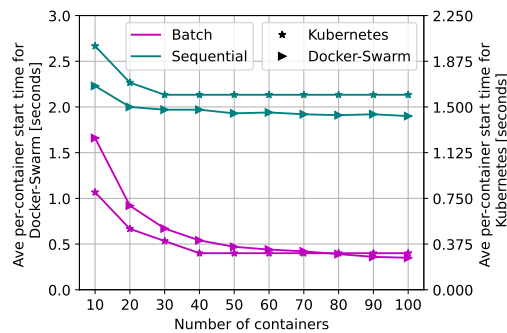
Fig. 4. Average per-container start-up time for batch and sequential deployment, using Kubernetes and Docker swarm.
