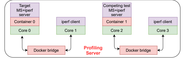
Fig. 1. Experimental testbed with target MS and competing MS.
