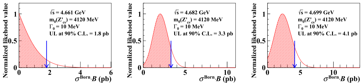
Fig. 4. (color online) Likelihood scan of \sigma^{\text{Born}} \cdot \mathcal{B} for the data samples at \sqrt{s} = 4.661, 4.682 , and 4.699 GeV after considering systematic uncertainties. The blue arrow indicates the upper limit at the 90% confidence level. In the likelihood scan, the PDFs which result in the largest upper limits are used, and the mass and width of Z'_{cs} are fixed to 4120 MeV/ c^2 and 10 MeV, respectively.
