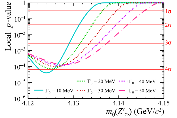
Fig. 6. (color online) The local p -value as a function of m_0(Z'_{cs}) from the simultaneous fit to data samples at \sqrt{s} = 4.661, 4.682 , and 4.699 GeV.
