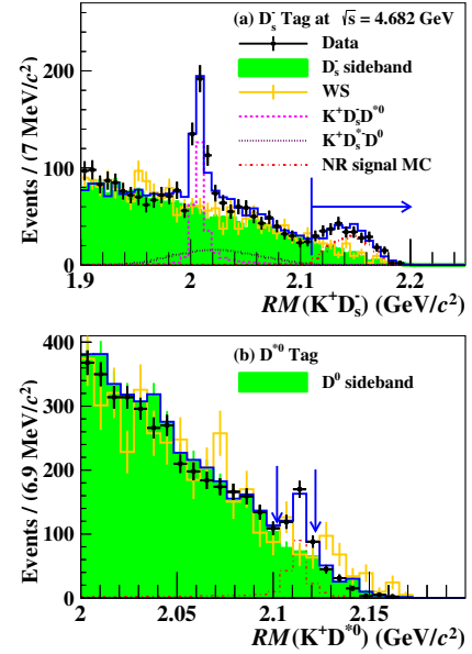
Fig. 2. (color online) The spectra of (a) recoil mass RM(K^+ D_s^-) of K^+ D_s^- and (b) recoil mass RM(K^+ D^{*0}) of K^+ D^{*0} for the D_s^- ( D^{*0} ) candidate events at \sqrt{s} = 4.682 GeV. The scaled background control samples of wrong sign (WS) events and D_{(s)} sideband events are overlaid to represent the combinatorial backgrounds. The scaled NR signal MC is also overlaid. The blue lines are the sum of spectra of scaled D_s^- sideband, e^+e^- \rightarrow K^+ D_s^- D^{*0} and e^+e^- \rightarrow K^+ D_s^{*-} D^{*0} and NR signal MC. The blue arrows indicate the selected region for the e^+e^- \rightarrow K^+ D_s^{*-} D^{*0} candidates.
