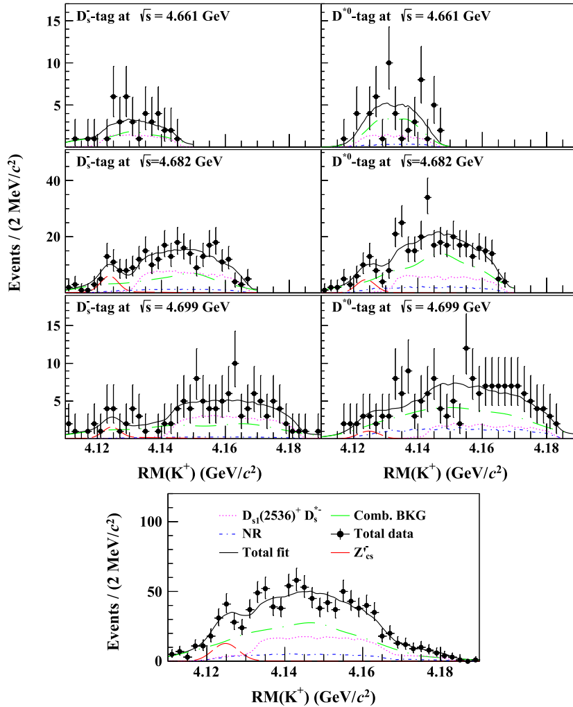
Fig. 3. (color online) The spectra of K^+ recoil mass from D^{*-} - and D_s^{*-} -tag methods after all selection criteria at \sqrt{s} = 4.661, 4.682 and 4.699 GeV. The simultaneous fit results are overlaid, where the red dashed lines are Z_{cs}^{\prime-} signals, the blue dashed-dotted lines are NR processes, the green dashed-dotted lines are combinatorial background, the purple dashed lines represent the process e^+e^- \rightarrow D_s^{*-}D_{s1}(2536)^+ and the black solid lines are the sum of all components.
