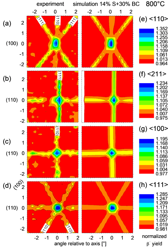
Figure 2: a)-d) Experimental \beta^- emission channeling patterns from ^{27}\text{Mg} in diamond around the \langle 110 \rangle , \langle 211 \rangle , \langle 100 \rangle , and \langle 111 \rangle directions during 800 °C implantation. The plots e)-h) are simulated theoretical patterns considering 14% on ideal substitutional and 30% on ideal bond-center sites.
