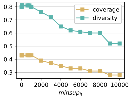
FIGURE 12. minsup_h sensitivity.
