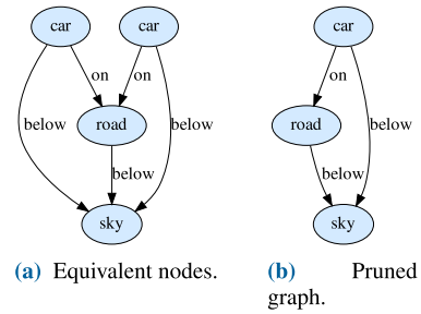
FIGURE 7. Node pruning.
