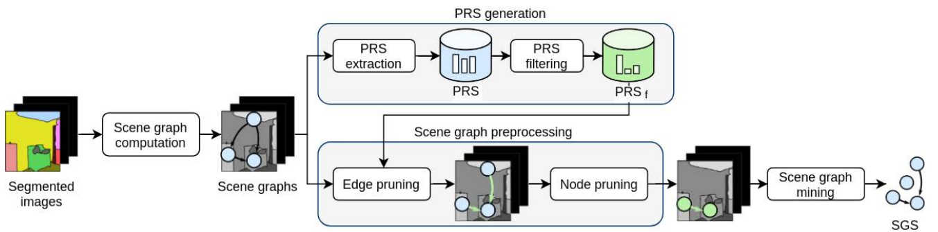
FIGURE 4. SImS architecture.
