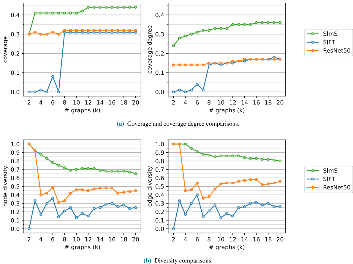
FIGURE 9. Quantitative comparison between SImS and KMedoids on COCO Subset 2 (garden-church, 890 images).
