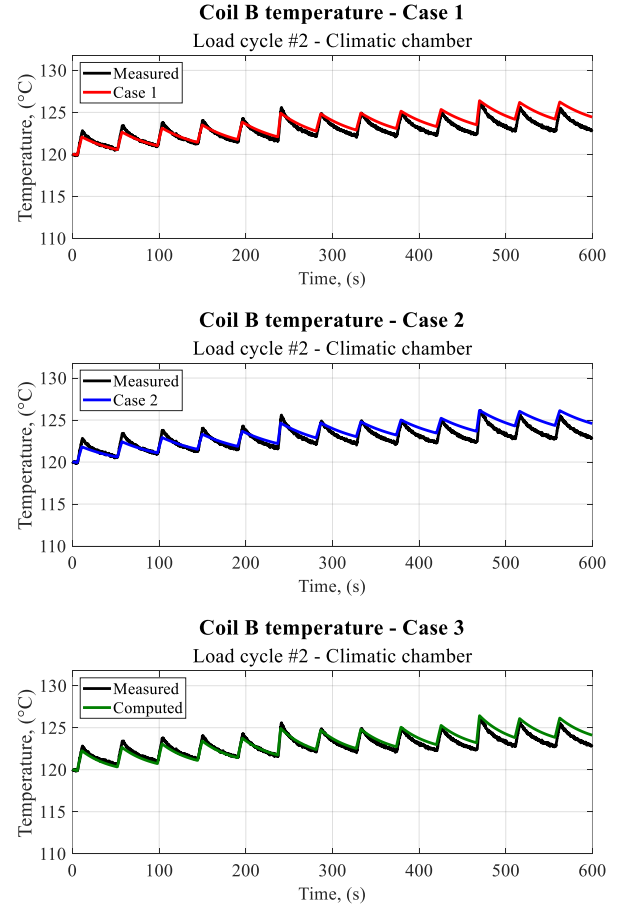
Fig.11 Measured and computed phase B temperature in the three cases of Table III for the two load cycles in the climatic chamber.
