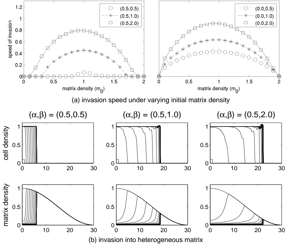
Figure 3: Top row: wavespeeds calculated for various different initial matrix densities, m_0 , and distinct (\alpha, \beta) pairs: (Left) wavespeeds for \alpha = 0.5 and \beta = 0.5 (dotted line/circles), \beta = 1.0 (dot-dash/stars) and \beta = 2.0 (solid/squares). (Right) wavespeeds for \alpha = 0.0 and \beta = 0.5 (dotted line/circles), \beta = 1.0 (dot-dash/stars) and \beta = 2.0 (solid/squares). Bottom row: Plots showing the invasion of cells (top row) into the spatially varying matrix (bottom row), with m(x, 0) = 0.5 + 0.5 \cos(\pi x/L) . In each frame, cell/matrix densities are plotted at increments of 10 between t = 0 and t = 200 . (Left) (\alpha, \beta) = (0.5, 0.5) , (Centre) (\alpha, \beta) = (0.5, 1.0) , (Right) (\alpha, \beta) = (0.5, 2.0) . Other parameters are set at L = 30 , L_i = 1.0 , n_0 = 0.1 , \gamma = 1 , K = 2.0 . Numerical details as in Figure 1.
