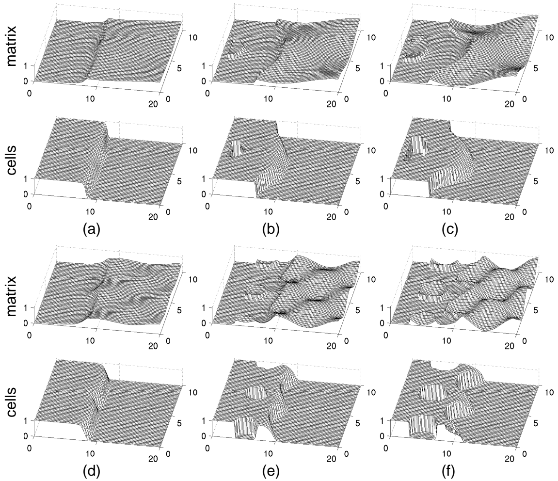
Figure 6: Invasion of cells into a “checkerboard” matrix. For each subfigure (a)-(f), plots represent matrix density (top) and cell density (bottom) plotted on the rectangular domain (x, y) \in [0, 20] \times [0, 10] at the fixed time t = 40 for the following initial matrix distributions: (a) m_0 = 0.5, m_1 = 0.1, k_y = k_x = 1 ; (b) m_0 = 0.5, m_1 = 0.3, k_y = k_x = 1 ; (c) m_0 = 0.5, m_1 = 0.5, k_y = k_x = 1 ; (d) m_0 = 0.5, m_1 = 0.1, k_y = k_x = 2 ; (e) m_0 = 0.5, m_1 = 0.3, k_y = k_x = 2 ; (f) m_0 = 0.5, m_1 = 0.5, k_y = k_x = 2 . Other model details as for Figure 5.
