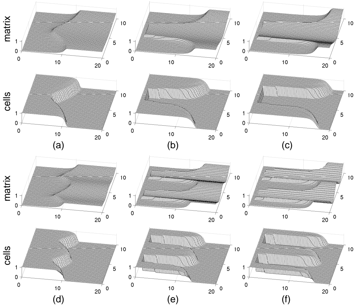
Figure 5: “Fingers” generated through invasion of cells into an initial matrix in which matrix density varies along the invasion front. For each subfigure (a)-(f), plots represent matrix density (top) and cell density (bottom) plotted on the rectangular domain (x, y) \in [0, 20] \times [0, 10] at the fixed time t = 40 for the following initial matrix distributions: (a) m_0 = 0.5, m_1 = 0.1, k_y = 1 ; (b) m_0 = 0.5, m_1 = 0.3, k_y = 1 ; (c) m_0 = 0.5, m_1 = 0.5, k_y = 1 ; (d) m_0 = 0.5, m_1 = 0.1, k_y = 2 ; (e) m_0 = 0.5, m_1 = 0.3, k_y = 2 ; (f) m_0 = 0.5, m_1 = 0.5, k_y = 2 . Model parameters are set as described in the text, (\alpha, \beta, \gamma, K) = (0.5, 1.0, 1.0, 2.0) , with n_0 = 0.1 and L_{id} = 1 .
