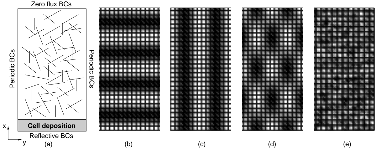
Figure 4: (a) Schematic showing the set-up for the 2D invasion model. (b)-(e) Representative plots of the initially imposed matrix densities as described in the text.
