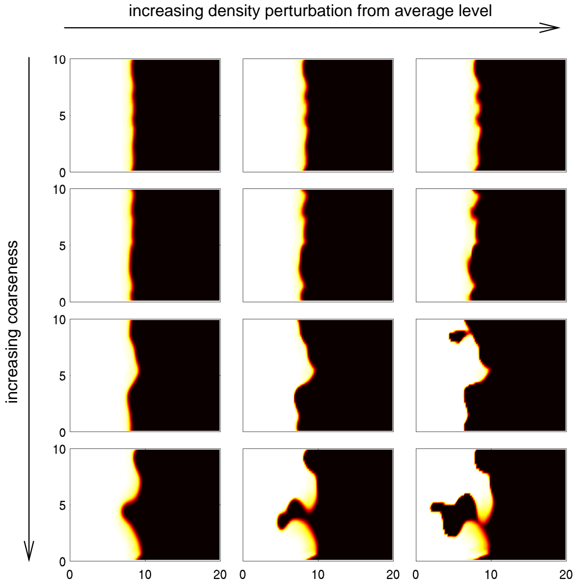
Figure 8: Cell invasion into various randomised initial matrices. Cell distributions plotted at t = 40 as density maps (white representing a density of 1, black representing a density of zero). Other model details as for Figure 5.
