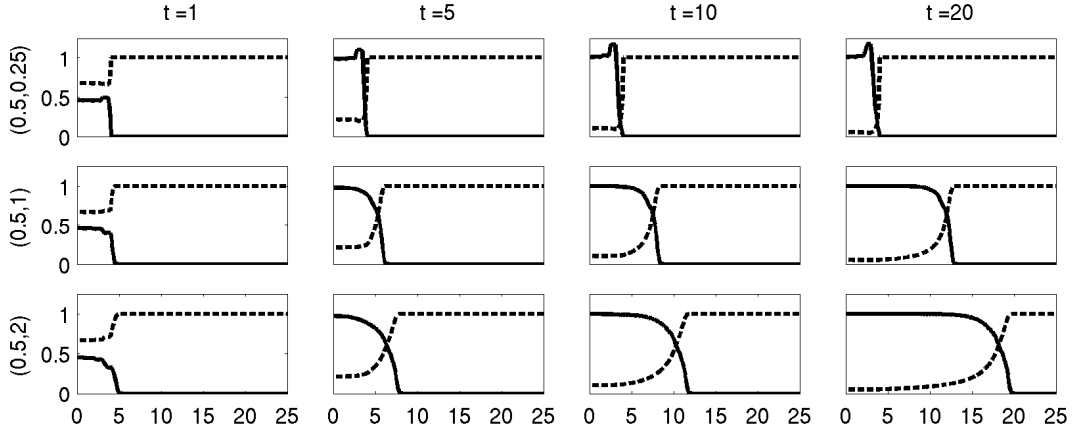
Figure 1: Non-invasive/invasive growth depends on the cell-cell:cell-matrix adhesive strength ratio. Rows plot cell density, n , (solid) and matrix density, m (dashed line) for various (\alpha, \beta) pairs: Top row, (\alpha, \beta) = (0.5, 0.25) ; Middle row, (\alpha, \beta) = (0.5, 1.0) ; Bottom row, (\alpha, \beta) = (0.5, 2.0) . Other parameters set at K = 2 , m_0 = 1 , n_0 = 0.1 , L_i = 4 and L = 40 (plots truncated at x = 25 for clarity of presentation).
