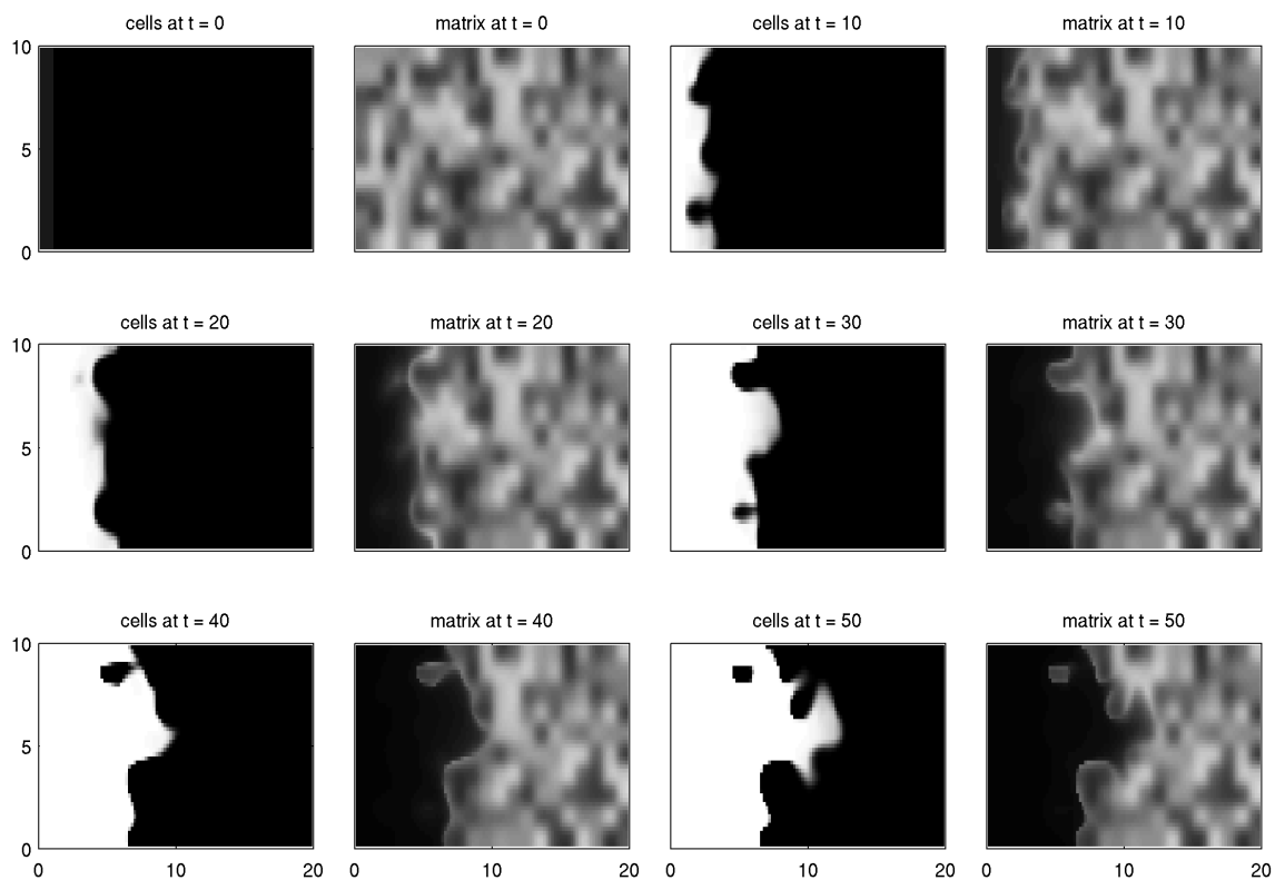
Figure 7: Time evolution of a cell invasion front into a “randomised” matrix structure. Cell ( n ) and matrix ( m ) densities are plotted at the various times shown, using a grayscale indicator (black indicating zero density and white representing a density of 1). Other model details as for Figure 5.
