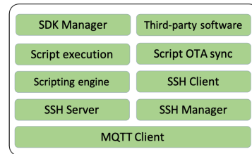
FIGURE 6. iottlyAgent architecture.
