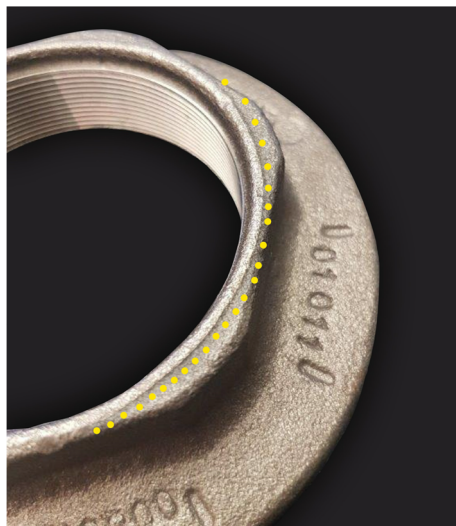
Fig. 5 Effects of elastic subsidence of the die on the forged part
