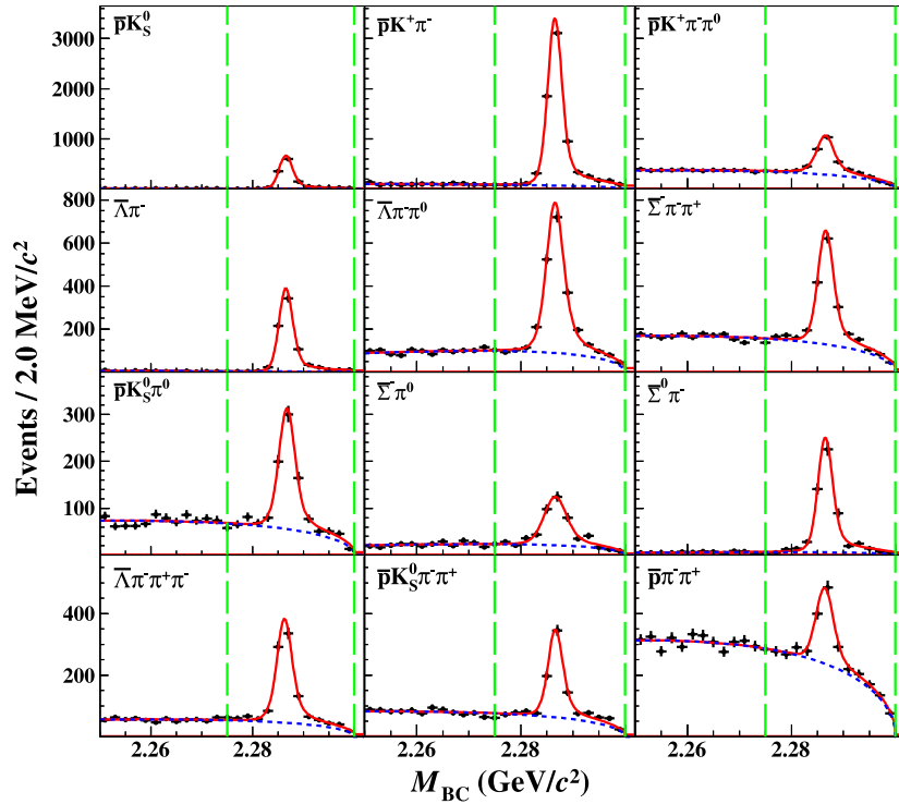
Fig. B1. (color online) The M_{BC} distributions of the ST \bar{\Lambda}_c^- candidates of various tag modes for the data sample at \sqrt{s} = 4599.53 \text{ MeV} . The points with error bars represent data. The red solid curves indicate the fit results and the blue dashed curves describe the background shapes. The ranges between green dashed lines are the signal regions.
