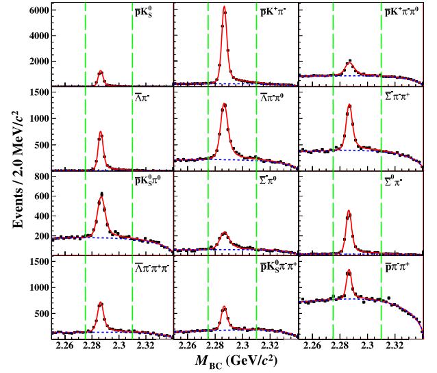
Fig. 2. (color online) The M_{BC} distributions of various ST modes for the data sample at \sqrt{s} = 4681.92 MeV. The points with error bars represent data. The (red) solid curves indicate the fit results and the (blue) dashed curves describe the fitted background shapes. The ranges between green dashed lines are the signal regions.
