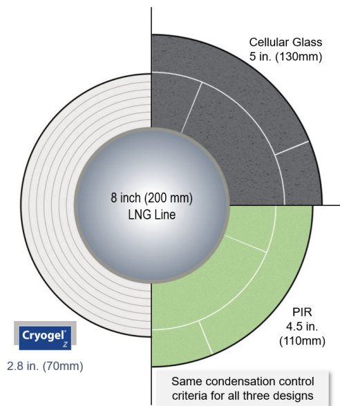
Figure 4: Cryogel Z. Source []
