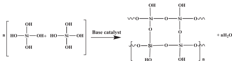
Figure 3. Silica Aerogel Synthesis with TEOS [35].
