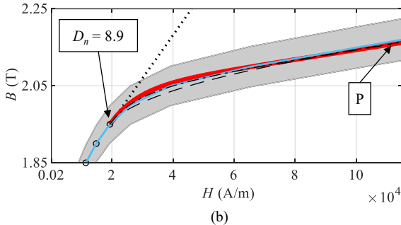
Fig. 5. The extrapolation of the reference curve (M36 steel) from medium field levels ( D_n = 8.9 ) to saturation using different strategies. (a) Detailed view and (b) zoom-in. The LAS and SEE methods are the most accurate ones. The QE method misestimates the value of the field in saturated conditions (point P).
