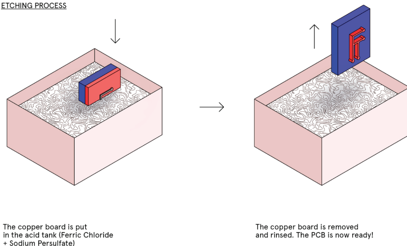
Figure 7. The subtractive method of etching a printed circuit board (our drawings)
