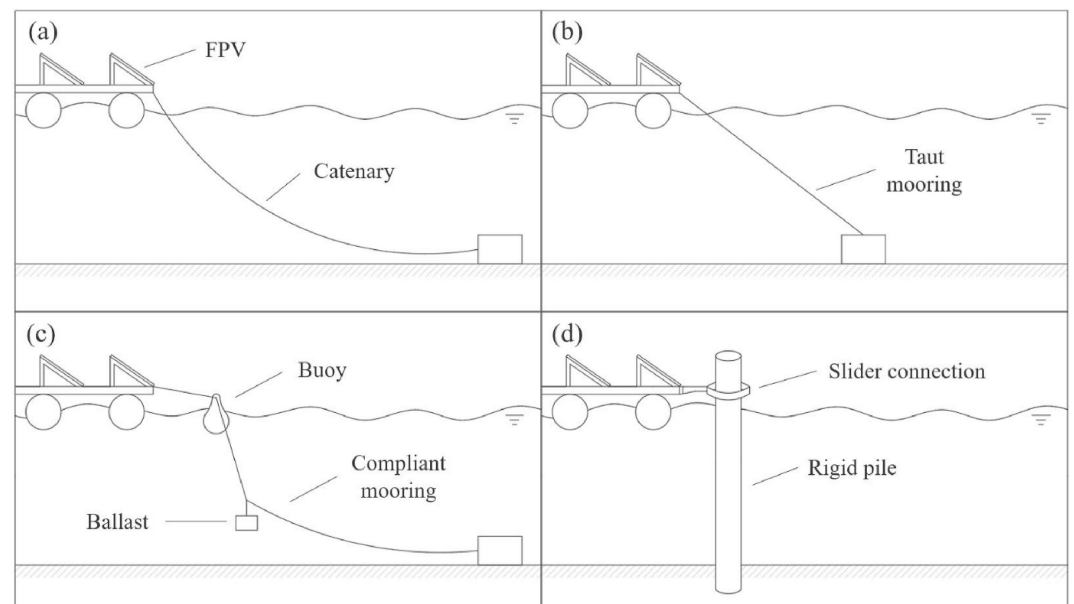
Figure 4. Mooring layouts: catenary (a), taut (b), compliant (c) and rigid (d) mooring, adapted from [25].
