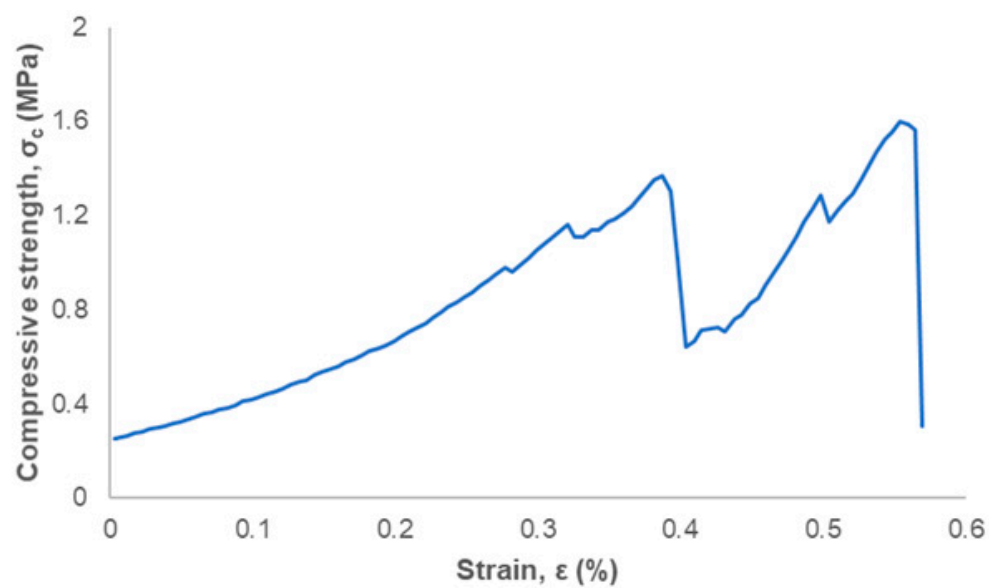
Figure 2. Typical stress–strain curve obtained after compressive test of hydroxyapatite scaffolds.
