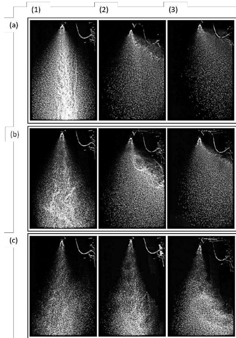
Figure 11. Lateralview of spray with hollowcone nozzle for (a) no rotor, (b) idle, and (c) throttle condition in (1) hovering, (2) at wind speed = 2 \text{ m}\cdot\text{s}^{-1} , and (3) at wind speed = 3 \text{ m}\cdot\text{s}^{-1} .
