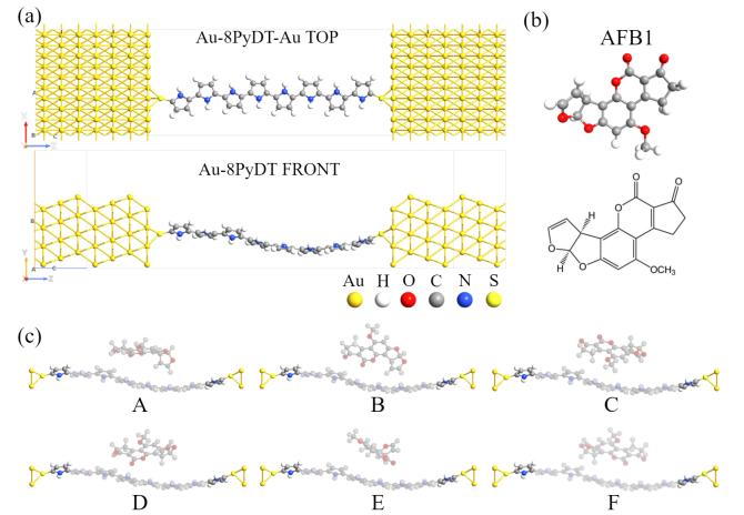
Fig. 1. (a) Top and front view of the Au-8PyDT sensor; (b) AFB1 molecule ( C4H4N8S2 ) and its structural formula; (c) The studied geometries with different relative orientations of AFB1 w.r.t. the Au-8PyDT after the geometry optimization. Bright atoms are fixed during the relaxation, while for the others no constraint is enforced.
