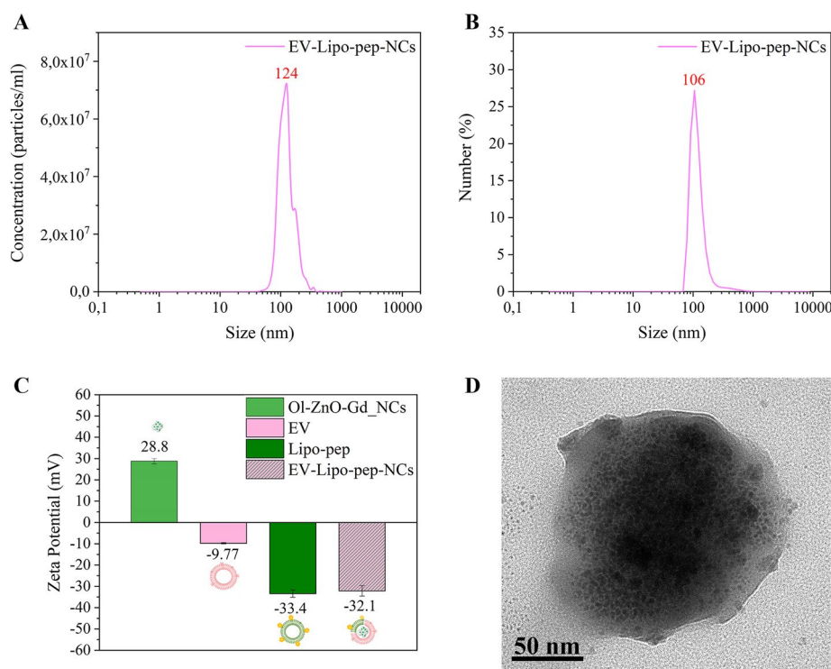
Fig. 4 Characterization of EV-Lipo-pep-NCs: size distribution resulting from A NTA and B DLS measurements of the EV-Lipo-pep-NCs nanoconstruct in a 1:1 solution of 0.1 \mu m filtered bidistilled water and 0.1 \mu m filtered 0.9% NaCl solution. C Comparison between zeta potential values of uncoated NCs, EVs, Lipo-pep, and EV-Lipo-pep-coated NCs. D TEM image at 60 kV of the nanoconstruct
