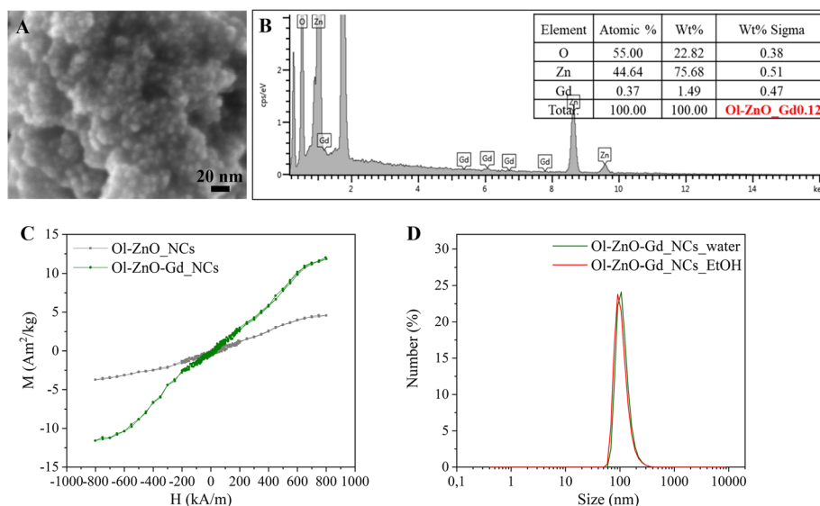
Fig. 2 Characterization of the Gadolinium-doped Ol-ZnO NCs: A field emission scanning electron microscopy (FESEM) image and B energy dispersive X-ray spectroscopy (EDS) confirming the successful inclusion of the dopant on the NCs prior to amino-functionalization (only O, Zn, and Gd were considered in the analysis). C Magnetization–saturation (M-H) curves comparing the magnetic behavior of amine-functionalized Ol-ZnO (gray curve) and Ol-ZnO-Gd (green curve) NCs. D Size distribution resulting from Dynamic Light Scattering (DLS) measurements of amine-functionalized Ol-ZnO-Gd nanocrystals in ethanol (red line) and water (green line)
