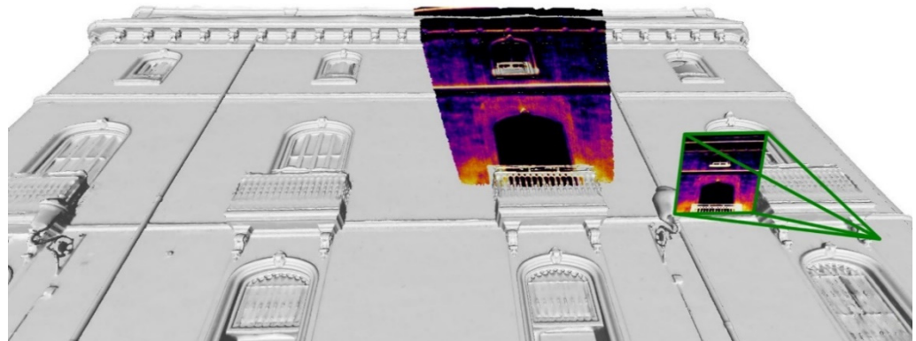
Figure 15. Projection of the TIR image evidencing a thermal discrepancy in the eastern façade, coherent with the presence of the remains of a previous frame of one of the main floor windows.
