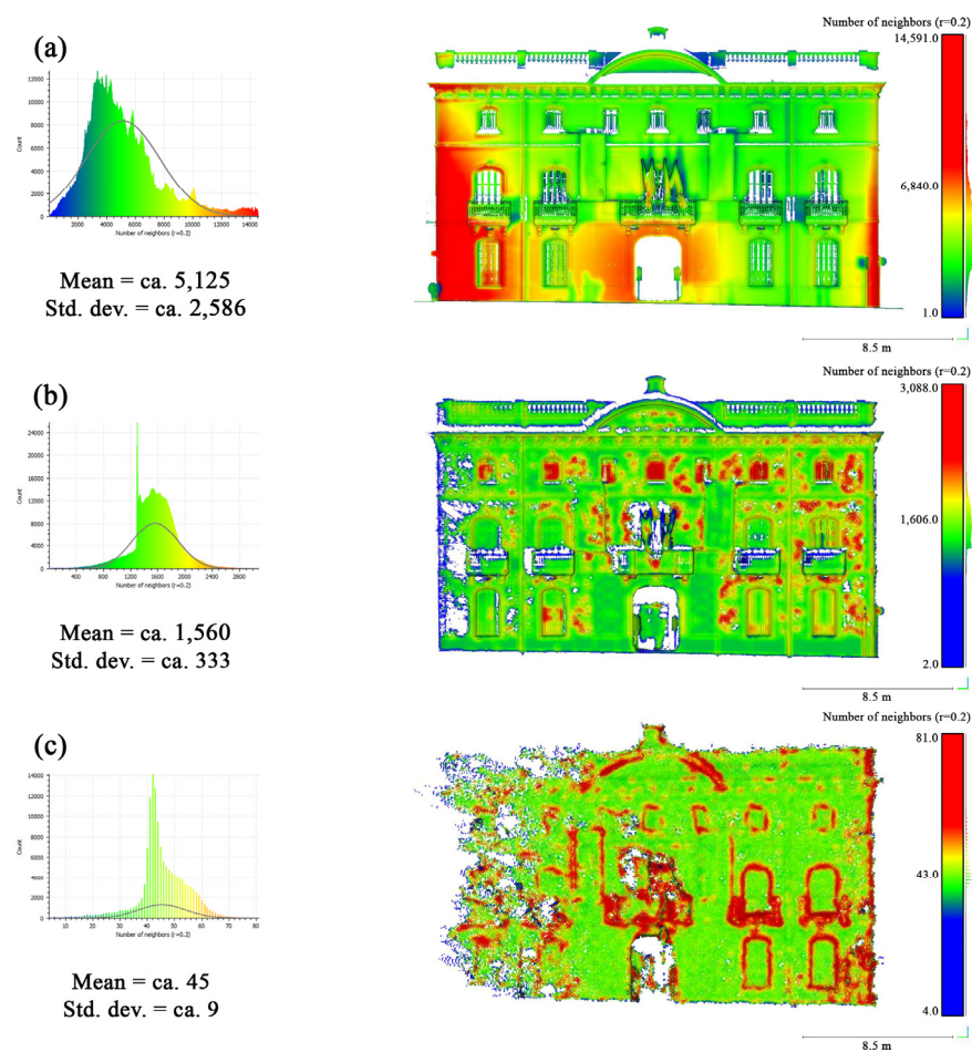
Figure 13. Density analysis. (a) LiDAR point cloud; (b) dense point cloud derived from colour images; (c) dense point cloud derived from TIR images.
