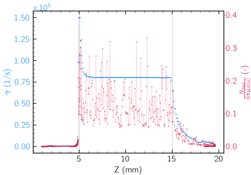
FIGURE 12 : Strain rate \dot{\gamma} (blue) and normalized maximum tensile stress N_{max} inside an isostatic cluster (red) along the Z -coordinate for a sample trajectory in the microchannel. The fluctuating behaviour of N is due to changes in the orientation of the cluster with respect to the flow field.
