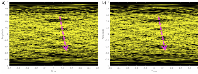
Fig. 4. Eyediagram of the noiseless channel output \bar{y}_{adc} transmitted at 50 GBaud over the transmission system a) obtained by Noise averaging acquisitions taken from the experimental setup b) obtained through simulation using the Multi-rate Channel model, previously trained using noiseless sequence \bar{y}_{adc} when transmitted at 58 GBaud in B2B.
