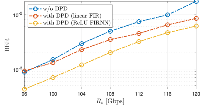
Fig. 8. BER vs Gross Bit Rate ( R_b ) curves obtained through simulation on the End-to-end system (B2B, L_{OPL}=8.5 dB). a) without DPD applied b) with linear FIR DPD applied c) with ReLU FIRNN DPD applied.
