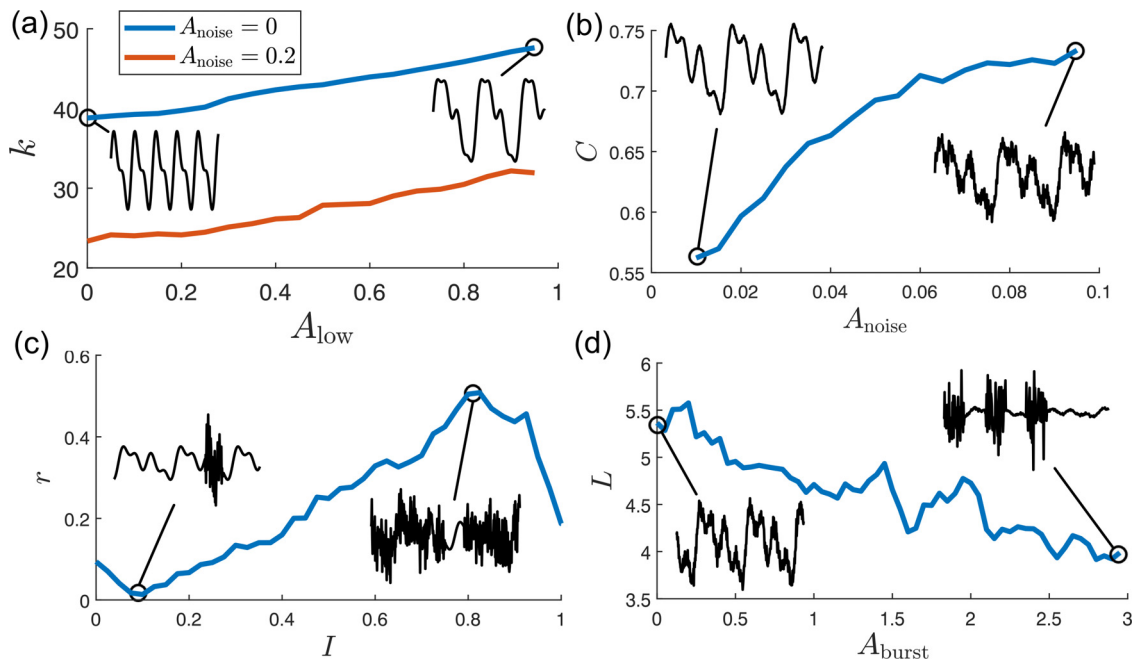
FIG. 3. Visibility parameters of the synthetic time-series: (a) average degree K with respect to the amplitude of the lowest frequency component of the time-series A_{\text{low}} ; (b) clustering coefficient C with respect to the amplitude of noise A_{\text{noise}} ; (c) assortativity r with respect to the intermittency I ; and (d) average path length L with respect to the amplitude A_{\text{burst}} of localized bursts ( I = 0.33 ). Relevant time-series are plotted as insets.
