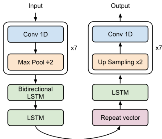
Fig. 2: Autoencoder architecture.
