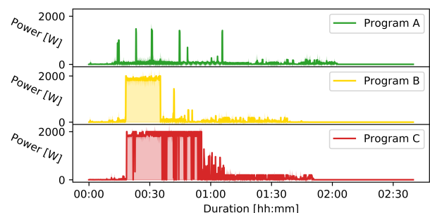
Fig. 4: Operational modes of the washing machine in the fourth house of the NILM dataset.
