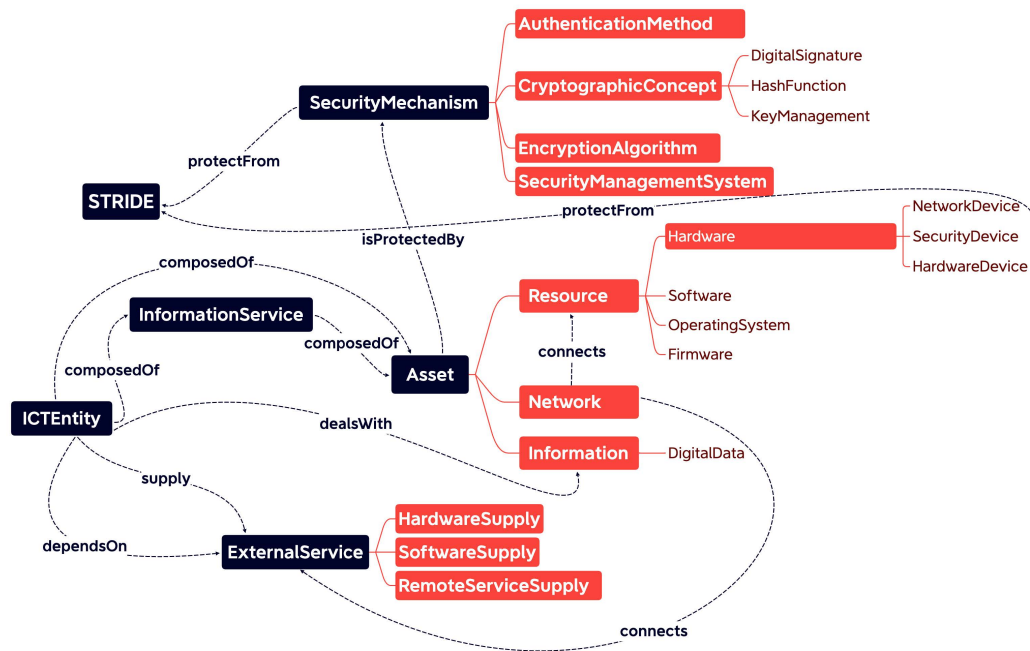
FIGURE 3. ICT sub-ontology.
