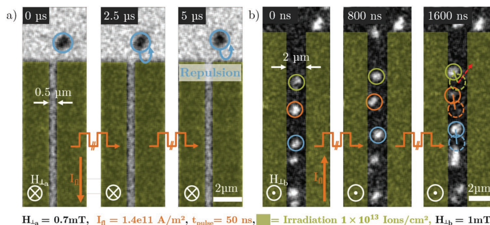
Figure 4. Two series of magneto-optical images of current-driven skyrmions. a) A track, exposed to an oop field of -0.7 \text{ mT} , that is composed of the untreated magnetic film while the surrounding barriers, indicated in transparent green, are irradiated with an FIB with high ion dose ( \approx 1 \times 10^{13} \text{ ions cm}^{-2} ). The same skyrmion after 0, 50 and 100, 50 ns-long current pulses with a current density of 1.4 \times 10^{11} \text{ A m}^{-2} (cumulative pulse time given in the images), is not able to enter the 500 \text{ nm} -wide track but is repelled from the irradiated areas. b) Three skyrmions, driven by current pulses (images after 0, 16 and 32, 50 ns-long pulses, current density 1.4 \times 10^{11} \text{ A m}^{-2} ), at a constant perpendicular field of 1 \text{ mT} . The skyrmions move straight along a 2 \mu\text{m} -wide track, formed by \text{Ga}^+ irradiation. The skyrmions move straight along the track as the heavily irradiated areas act as a repulsive barrier, counteracting the motion due to the Magnus force. In the final image, the beginning and end positions of the skyrmions are indicated to visualize the straight motion along with the hypothetical free motion of a skyrmion in red.
