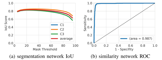
Fig. 8. Networks performances in terms of IoU score and mask threshold in (a) for the semantic segmentation model, and receiver operating characteristic curve in (b) for the similarity-based neural network.
