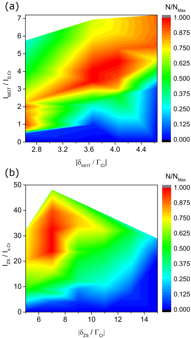
FIG. 5. (a) Steady-state MOT population, rescaled to its optimum value, as a function of both the normalized single-beam peak intensity I_{MOT}/I_{S,Cr} and the detuning |\delta_{MOT}/\Gamma_{Cr}| of the cooling light, see color code on the right. This measurement employs a radial MOT gradient of 12.6 G/cm, and a ZS beam intensity (detuning) of 32 I_{S,Cr} ( -7\Gamma_{Cr} ). (b) Same as panel (a) but for the ZS cooling beam parameters. The given ZS beam intensity corresponds to the one estimated at the MOT region. For this measurement, the single MOT beam peak intensity (detuning) is set to 3.5 I_{S,Cr} ( -3.5\Gamma_{Cr} ).
