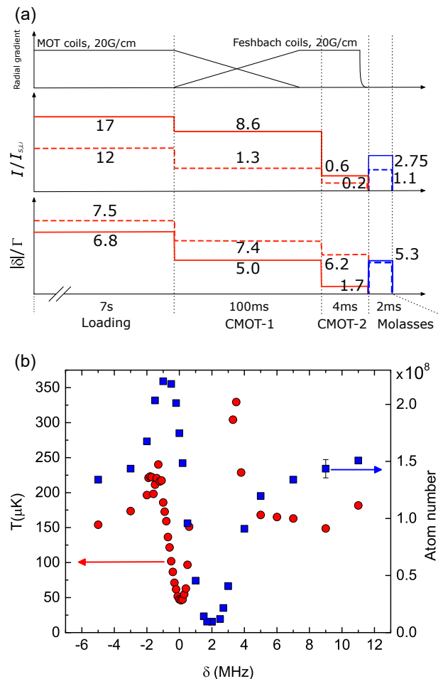
FIG. 4. (a) Sketch of the experimental routine employed to produce cold clouds of 6 Li atoms in our experiment. For each stage, red (blue) solid and dashed lines indicate the parameters exploited for D_2 ( D_1 ) cooling and repumper lights, respectively. The transfer from the MOT coils to the Feshbach coils quadrupole is also shown by the black solid lines. (b) Temperature (red circles, left axis) and atom number (blue squares, right axis) as a function of the relative detuning \delta of the D_1 repumper and cooling lights, recorded after 2 ms of gray molasses. At the Raman condition, \delta = 0 , a minimum temperature of 45(5) μK is obtained, with a cooled fraction N/N_0 \sim 70\% . For this measurement, the total cooling and repumper peak intensities were fixed to the optimum values I_{cool} = 2.75 I_{S,Li} and I_{rep} \sim 0.4 I_{cool} , respectively.
