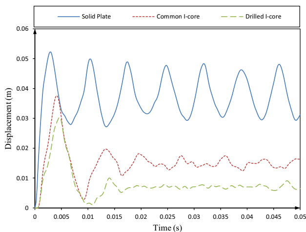
Fig. 12 Time-history of midpoint displacement under 3 kg TNT
