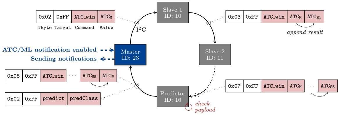
Fig. 4. I 2 C protocol communication example during ATC and ML modes working concurrently: the master board sends the ATC.win command (attaching its TC count as first payload's value) to request for the ATC values of all the boards; the predictor, after checking the payload's dimension, firstly attaches its TC count to return the ATC I 2 C packet to the master, then predicts the gesture and closes the loop sending the recognition result.
