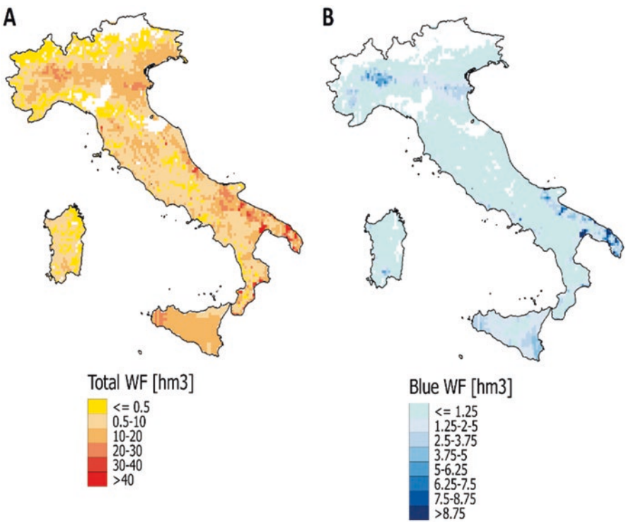
Fig. 13.5 The Italian water footprint at 5'x5' resolution referred to year 2010: blue plus green water footprint (a), blue water footprint (b)
