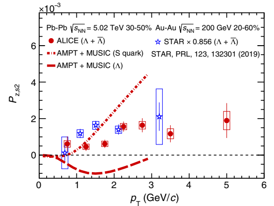
FIG. 3. Transverse momentum dependence of P_{z,s2} averaged for \Lambda and \bar{\Lambda} in Pb-Pb collisions at \sqrt{s_{NN}} = 5.02 TeV in semi-central collisions and its comparison with the similar RHIC results for Au-Au collisions at \sqrt{s_{NN}} = 200 GeV. The model calculations [38] for \Lambda and strange quark for Pb-Pb collisions at \sqrt{s_{NN}} = 5.02 TeV in the 30%–50% centrality interval using the approach described in Ref. [23] are shown by dash-dotted lines.
