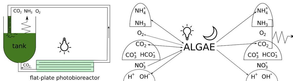
Figure 1: left) Schematization of the lab-plant for microalgae growth. Nutrients are added at the process start-up. CO 2 is supplied at the tank exit. Gaseous species are released to the atmosphere from the liquid free surface. Right) Graphical representation of the components considered by the kinetic model. Arrows indicate species that are either consumed or produced, or both, by the microalgae. The bells group species in chemical equilibrium with each other.
