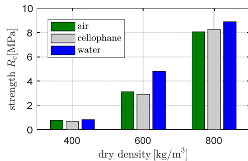
Fig. 7 Effect of curing conditions on the achievement of the compressive strength (CEM IV/A 42,5R, w/c = 0.3 )
